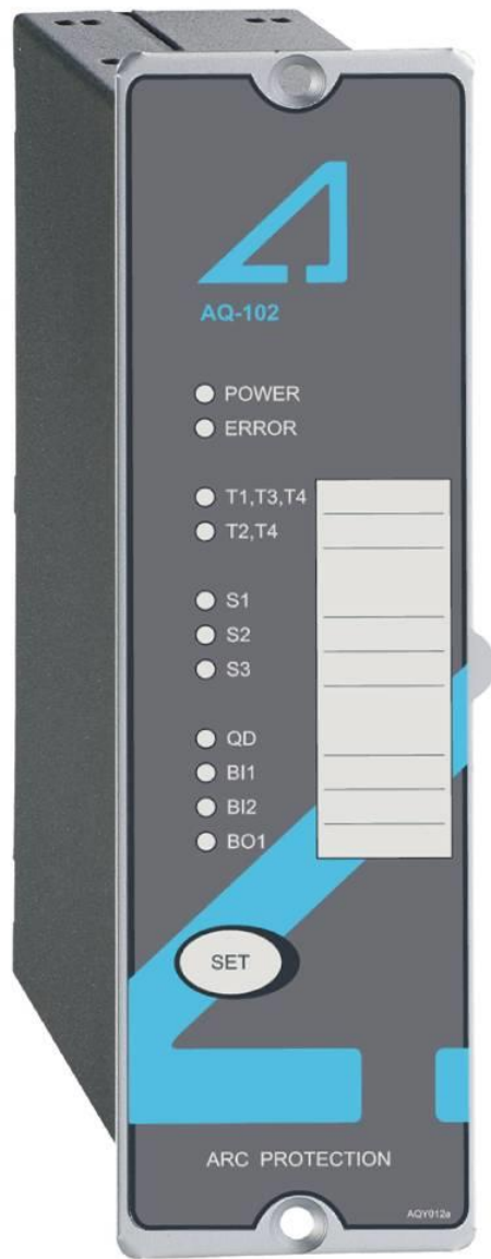
Figure 2-1 Arc protection unit AQ 102
