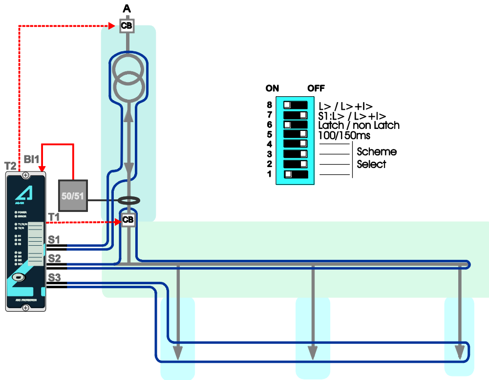
Figure 6-1: LV or MV stand-alone application.
