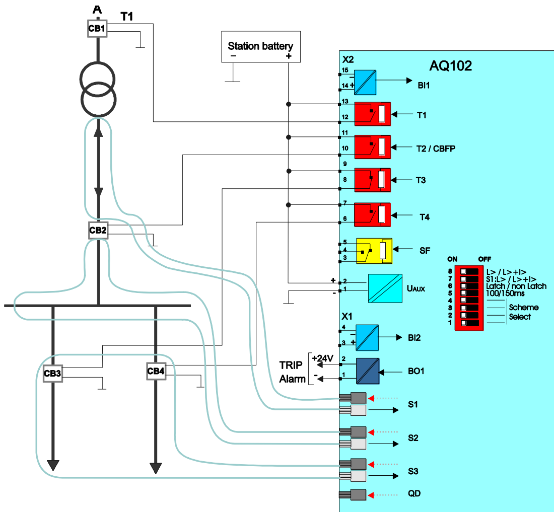
Figure 8-1: Wiring diagram of AQ102 unit.
