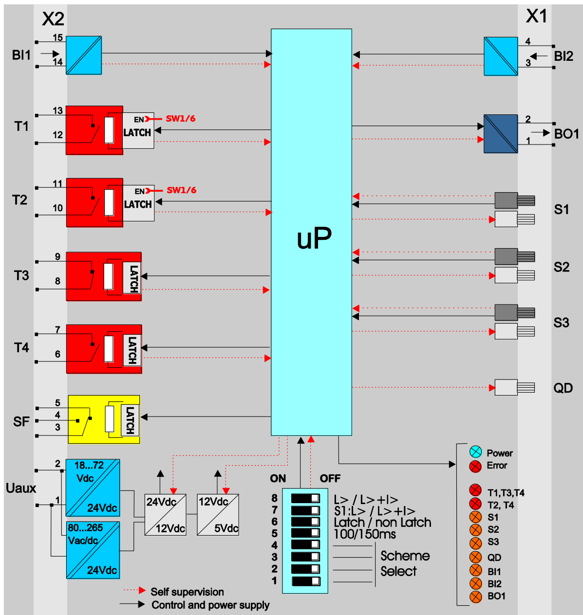
Figure 2-2 AQ 102 simplified block diagram
