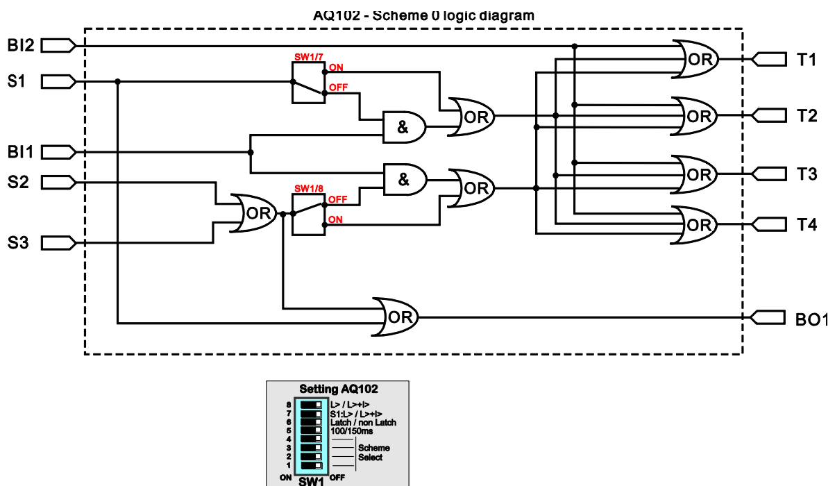
Figure 3-2: AQ102 logic scheme 0
