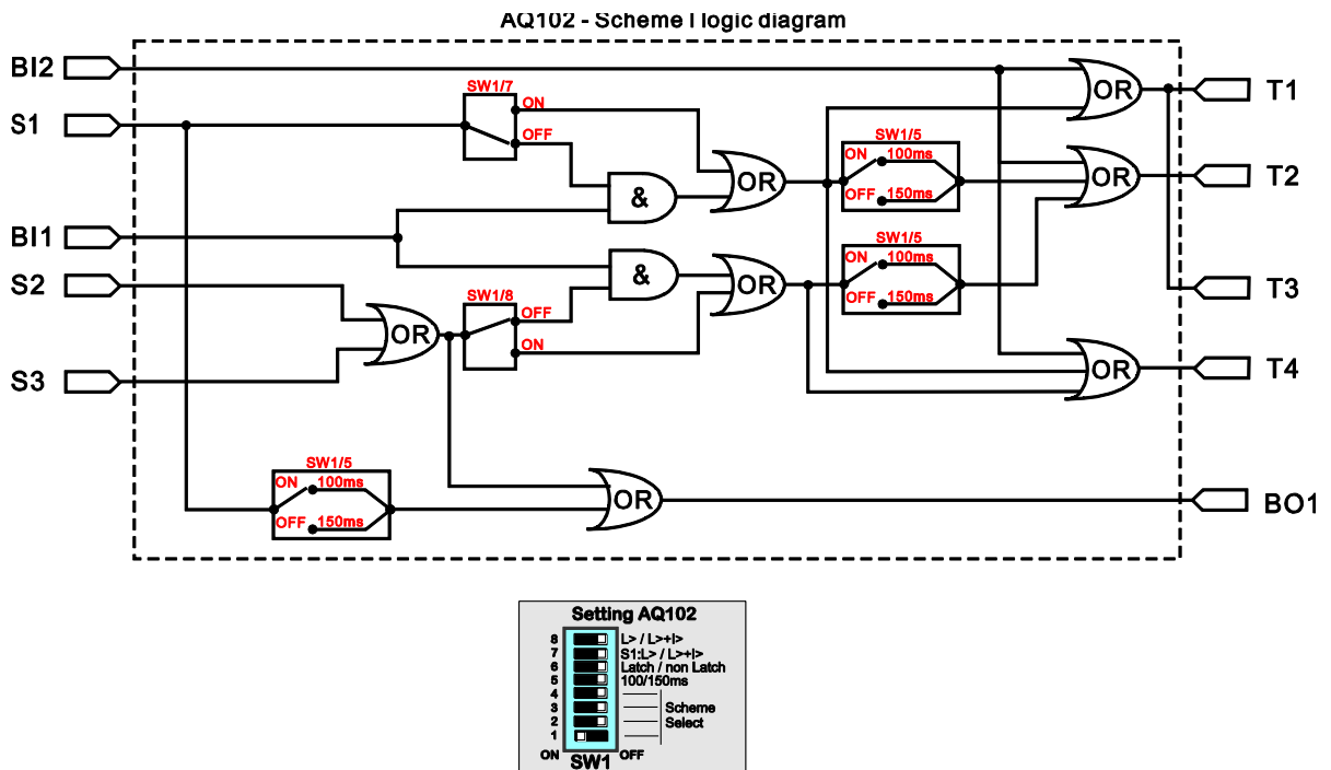
Figure 3-3: AQ102 logic scheme I
