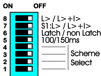
Figure 3-1 AQ 102 dipswitches
